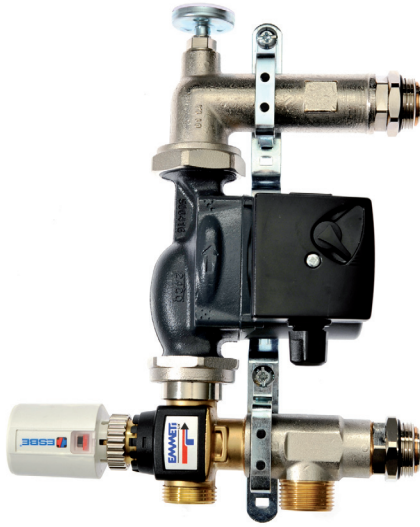
Alternative T3 control set with electrothermic actuator, U9 700 030
