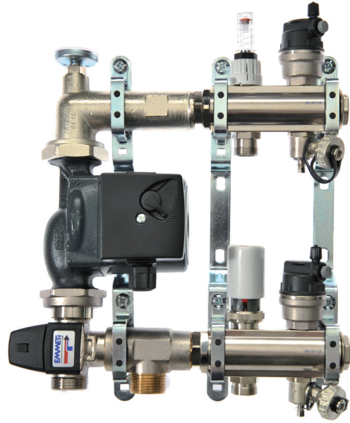
Single Loop Manifold with T3 control set, U9 700 020
